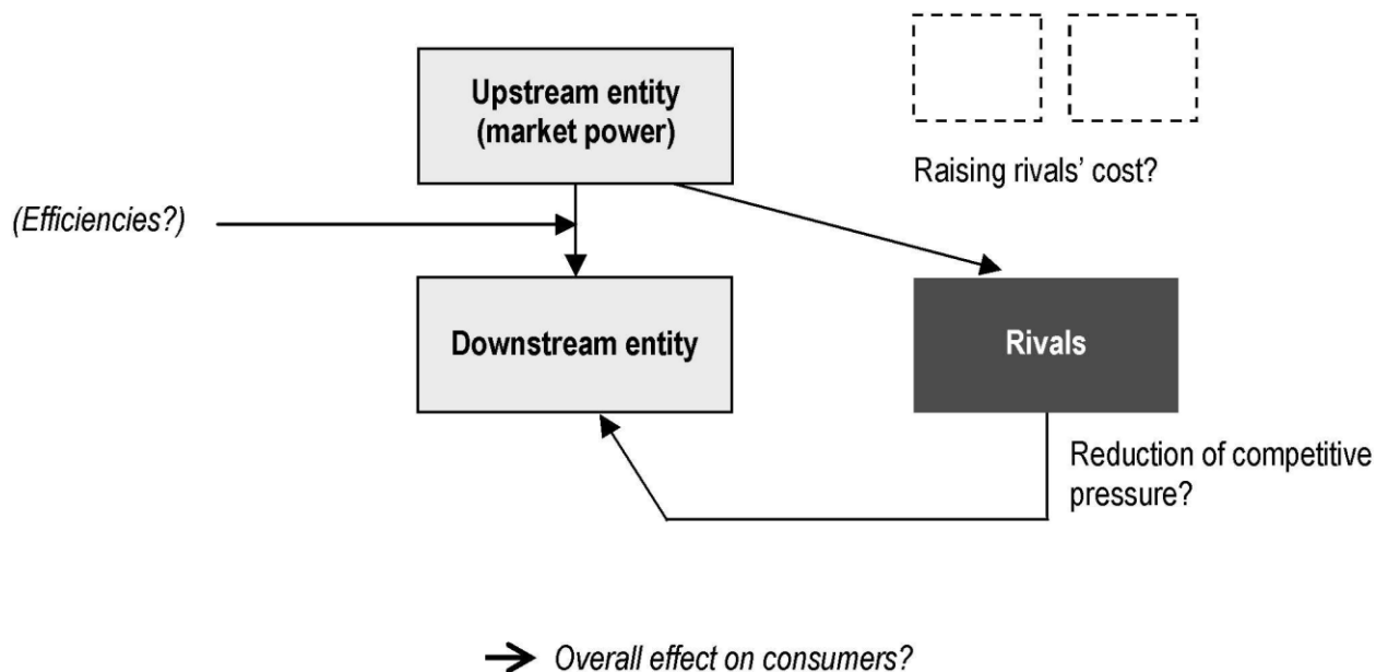
Figure 1 - Input foreclosure
