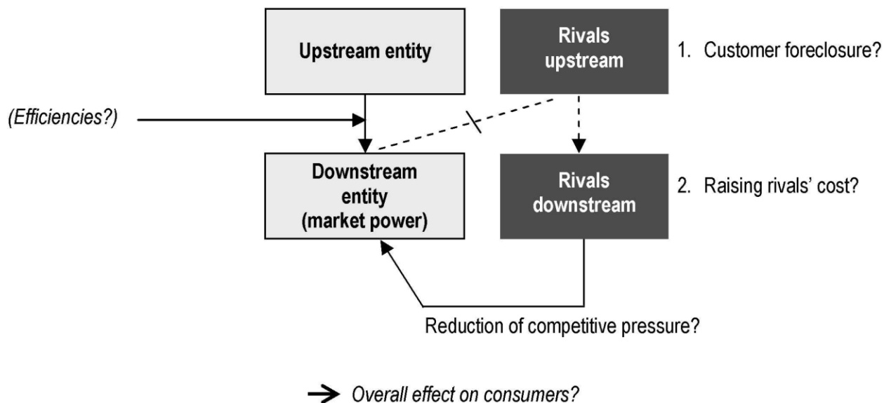
Figure 2 - Customer foreclosure
